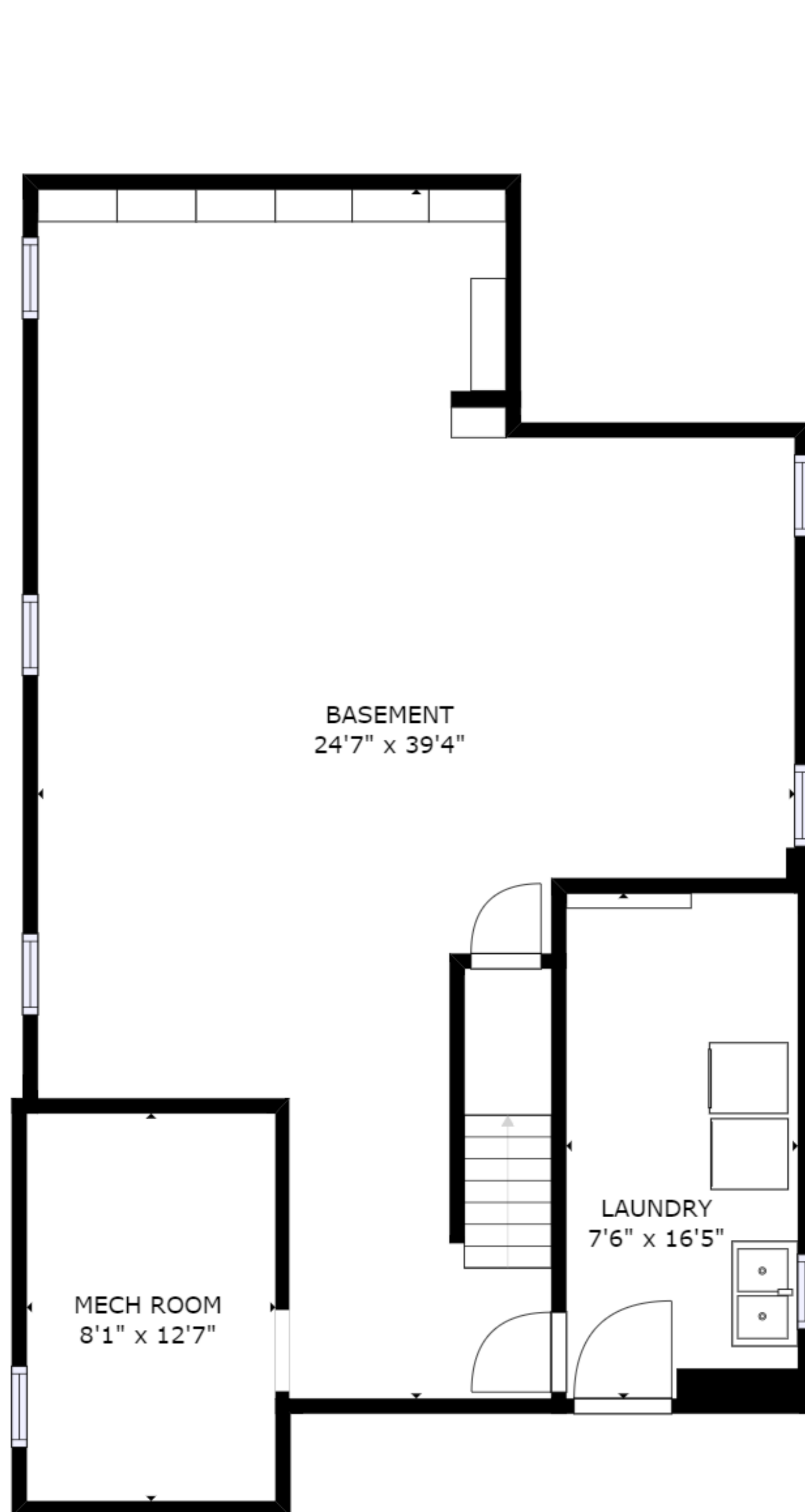
FLOOR 1
