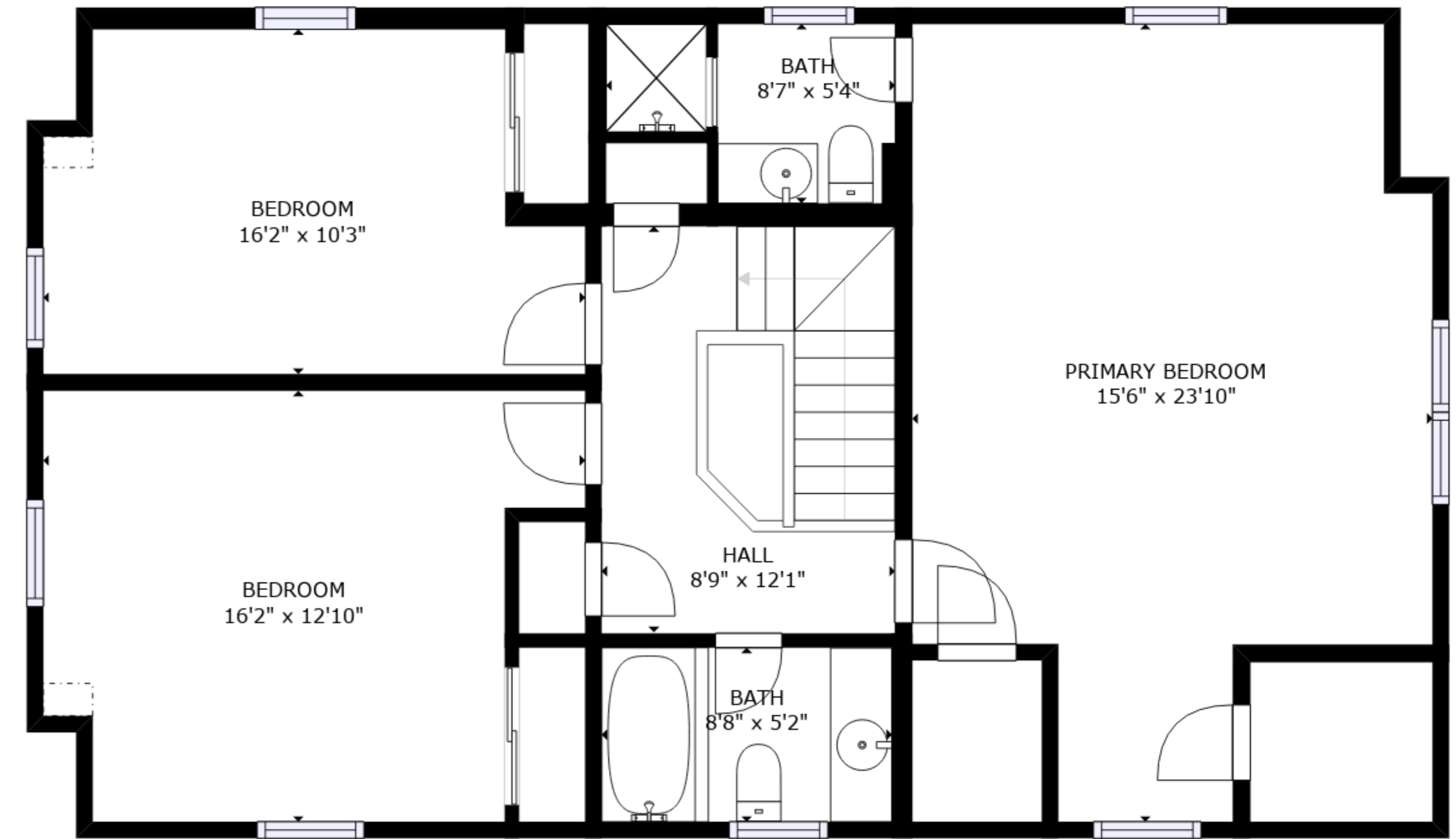
FLOOR 3
