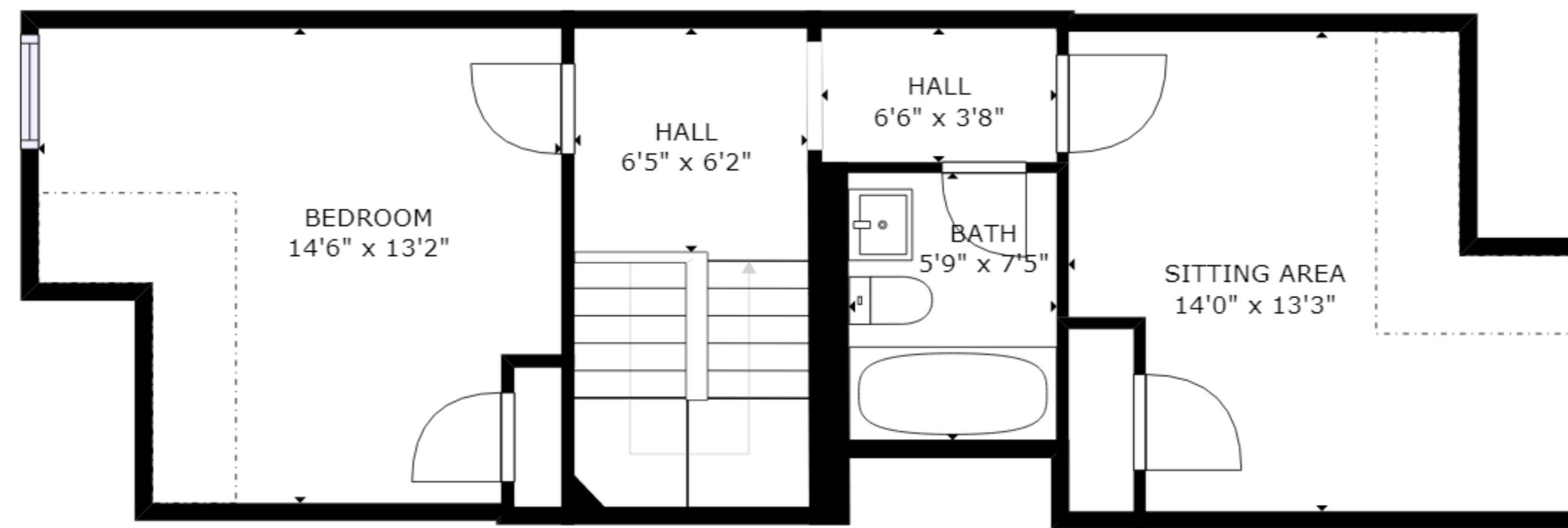
FLOOR 4
